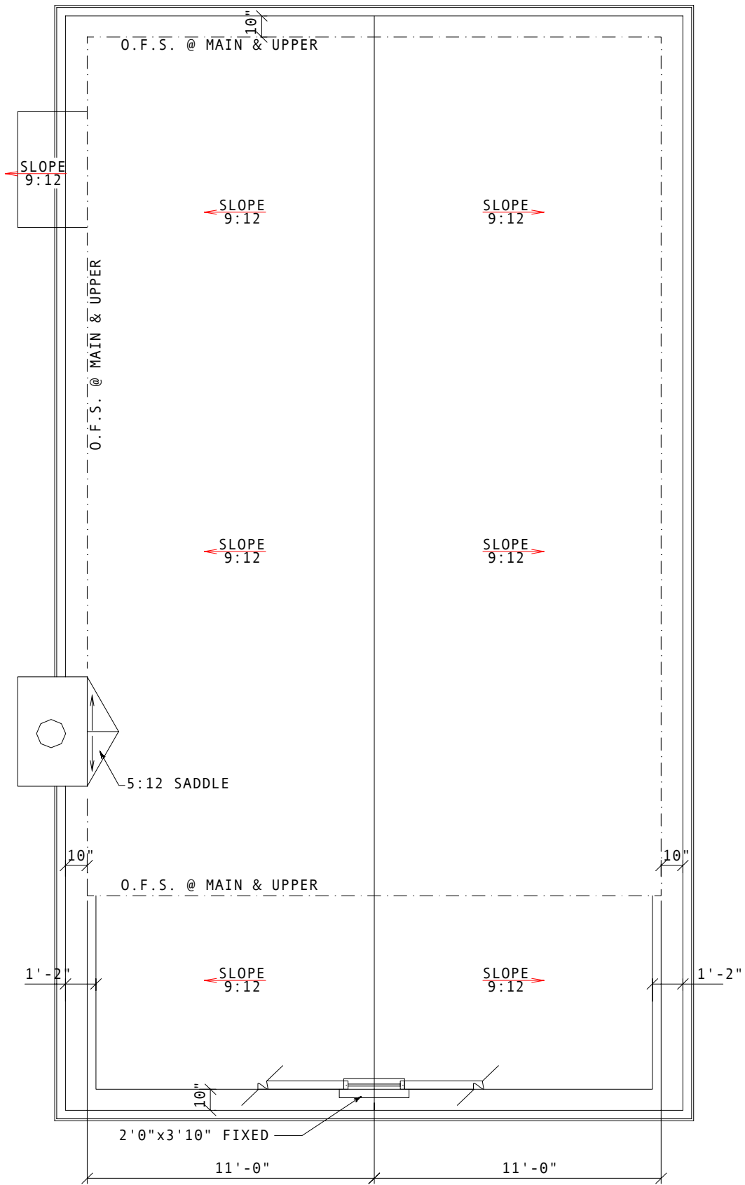
Roof Plan
