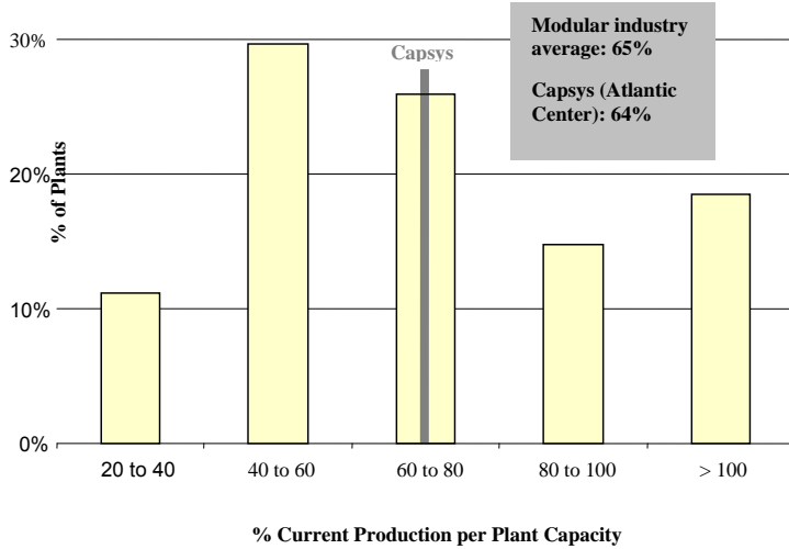
Figure 17 Capacity utilization
