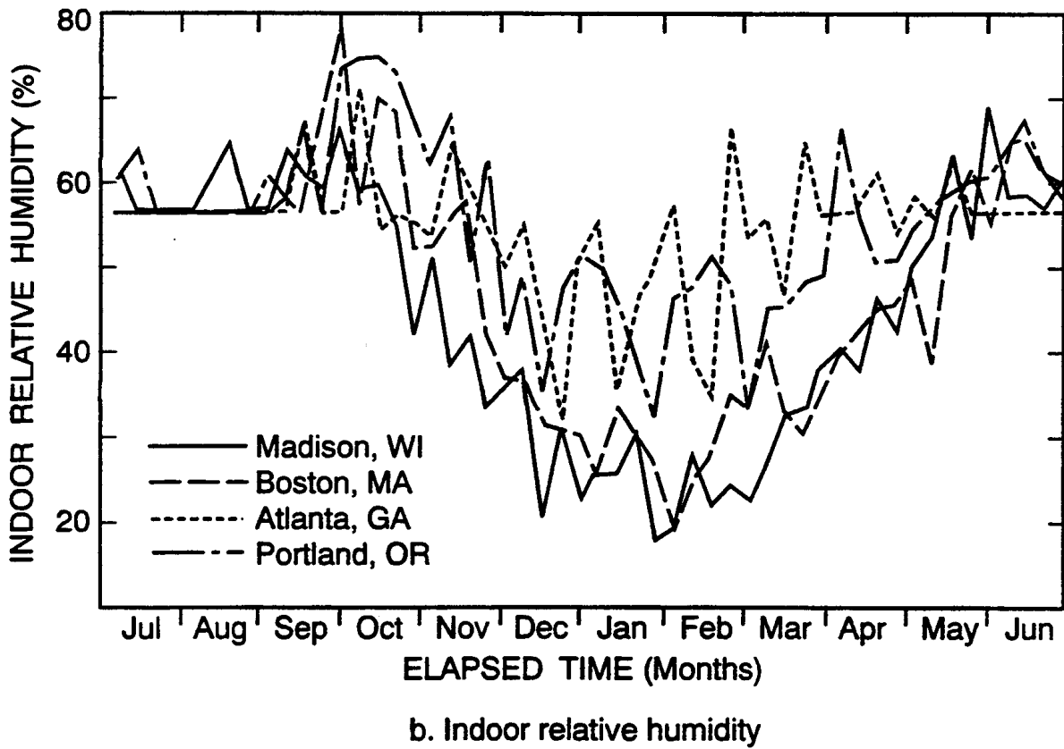
Fig. 16. Effect of outdoor climate on the surface moisture content of north-sloping plywood roof sheathing and indoor relative humidity for current practice house.
