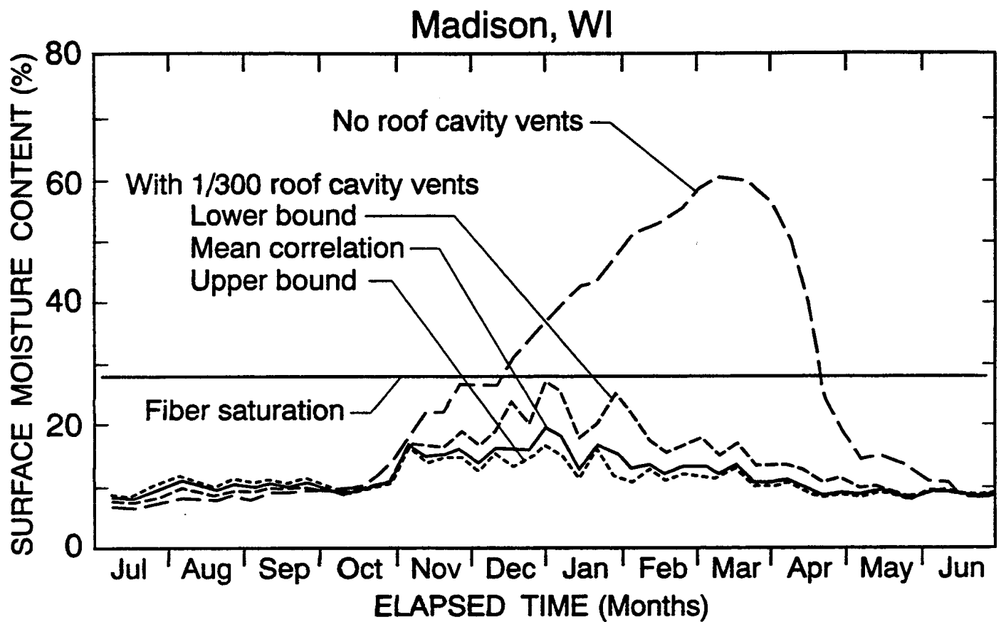
Fig. 19. Effectiveness of roof cavity vents in tight house with high moisture production rate.
