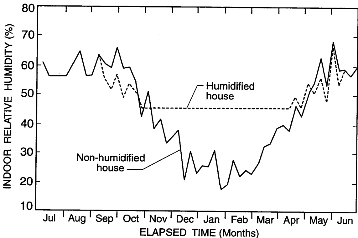
b. Indoor relative humidity
