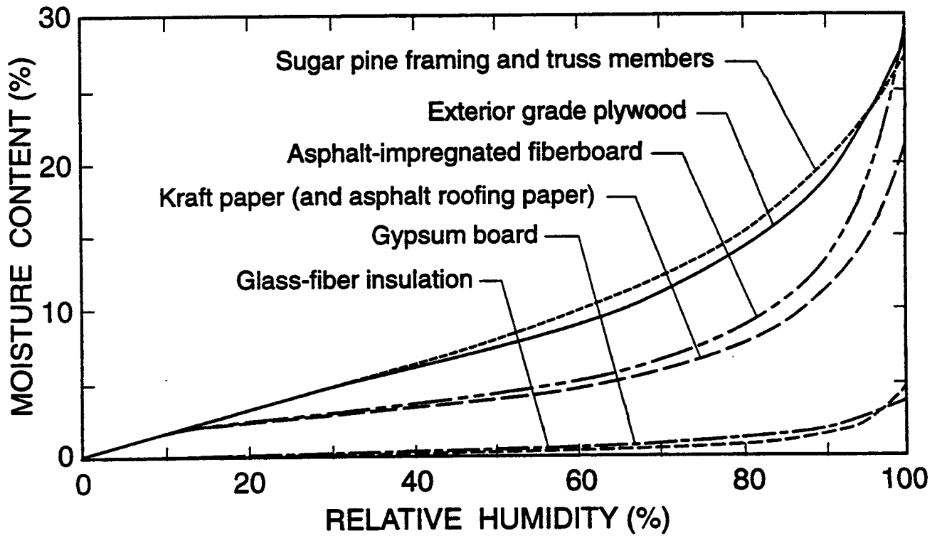
Fig. 4. Sorption isotherms of the materials.
