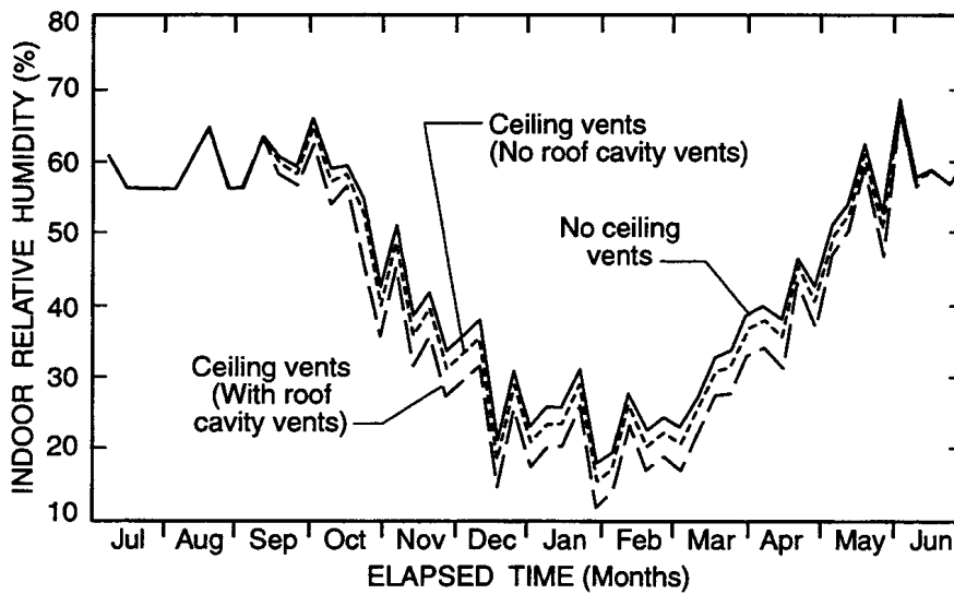
c. Indoor relative humidity
