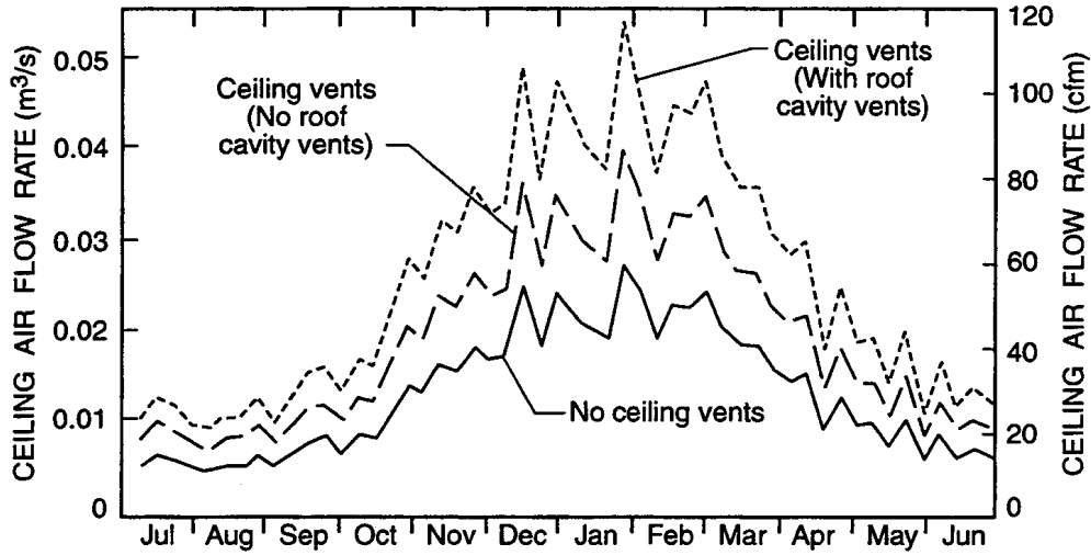
b. Airflow from house into roof cavity
