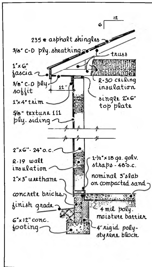
Figure 6. Typical Wall Section
