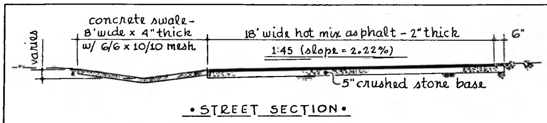
Figure 2. Street Section
