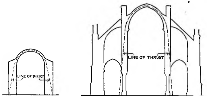
FIG. 52—THE ARCH THRUST
