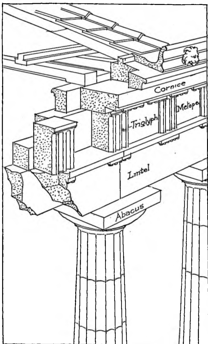
FIG. 8—GREEK STONE CONSTRUCTION
