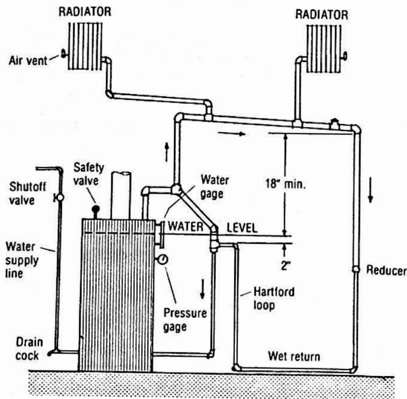
One-pipe steam heating system.
