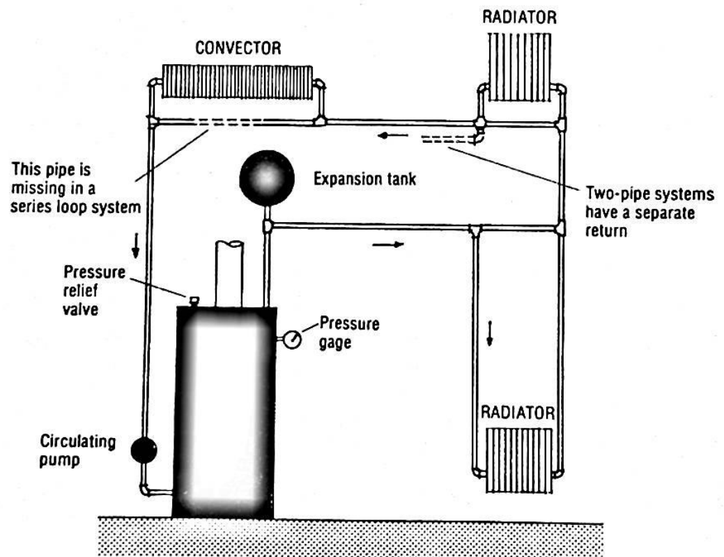
One-pipe forced hot water heating system.
