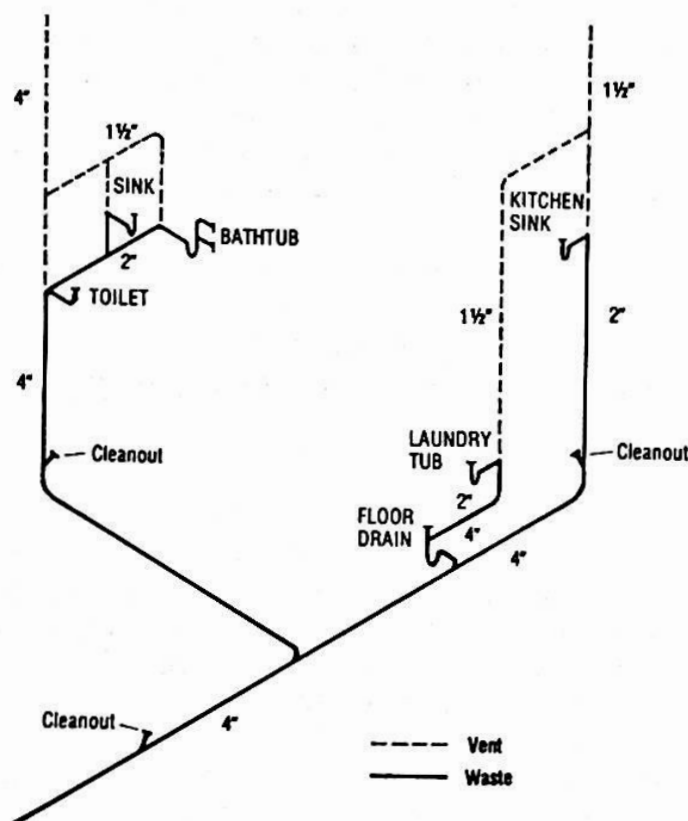
Typical drain, waste, and vent (DWV) piping schematic for a single family residence.
